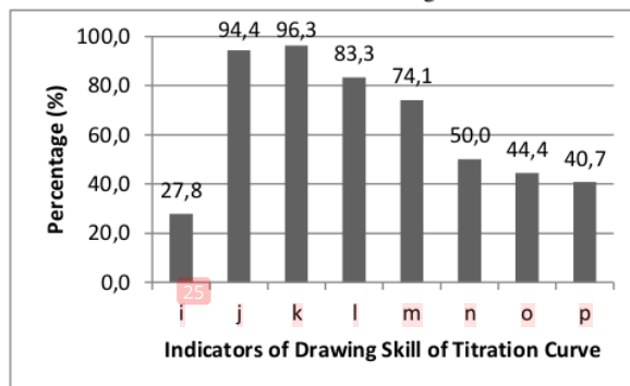
Figure 3. Level of drawing skills of titration curve.
