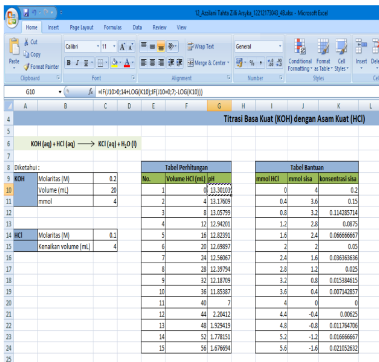
Figure 2. The calculation and a help table of drawing skills titration curve.
