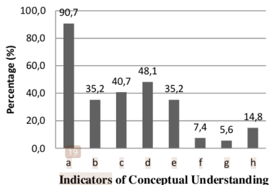
Figure 1. Level of conceptual understanding of acid-base titration.
